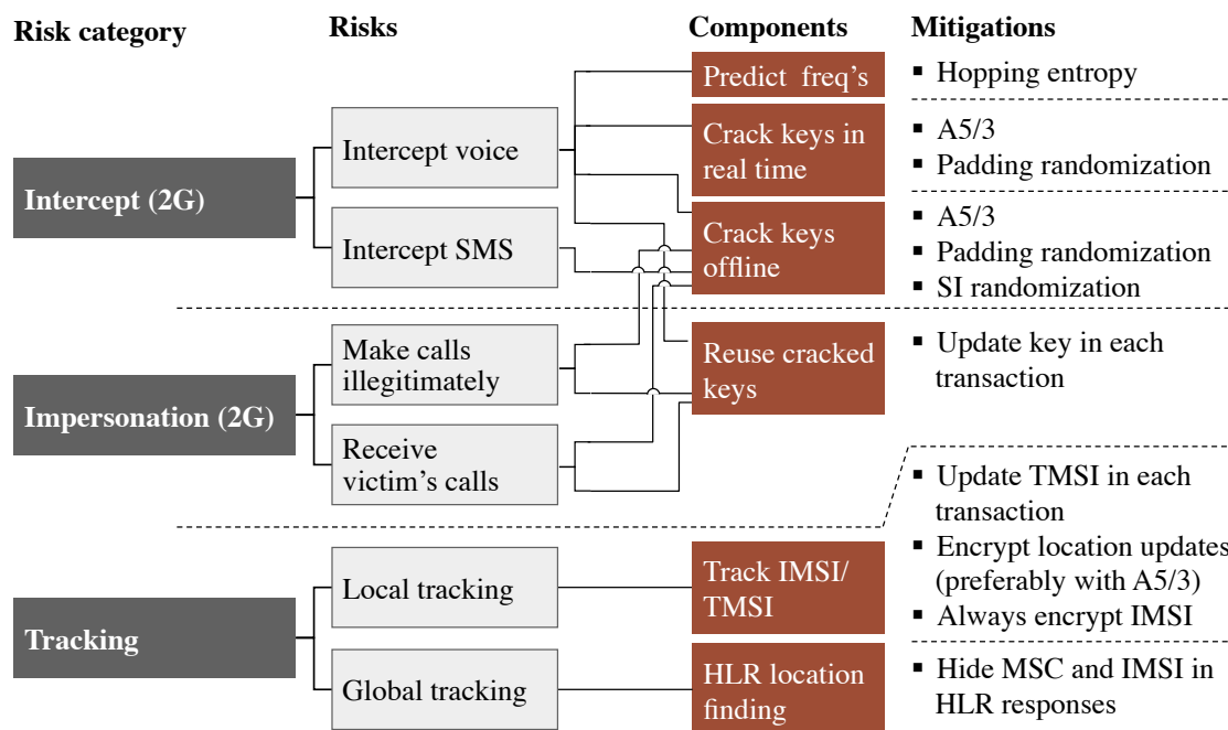
Figure 1: Best practice protection measures can mitigate three attack scenarios.
